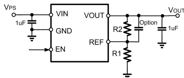
Figure 1B, Typical Application Circuit of AS9195 Adjustable Output Voltage ( V_{REF}=1.8V )
