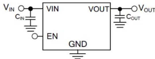
Figure 1A, Typical Application Circuit of AS9195 Fixed Output Voltage
